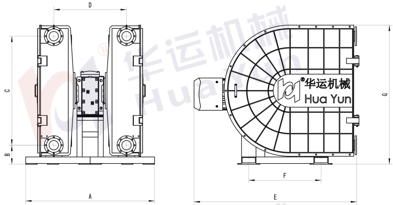
Products dimension
